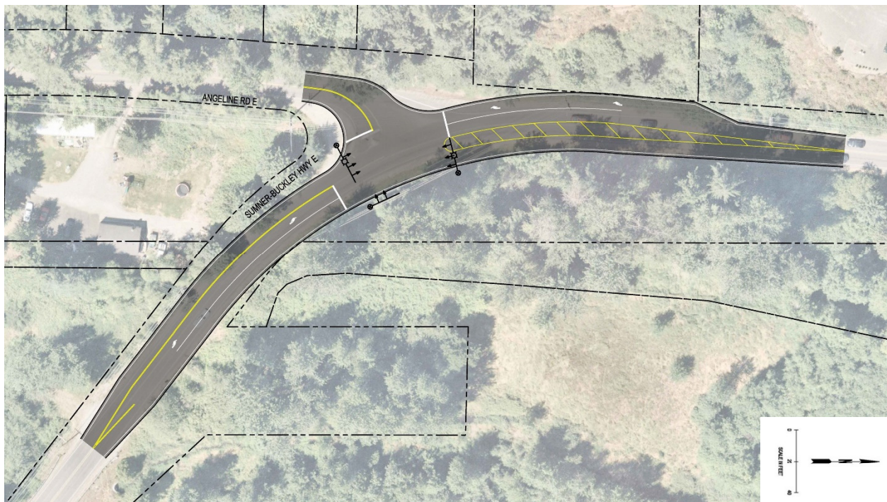
Figure 9. Angeline Road at Veterans Memorial Drive - Traffic Signal Alternative
