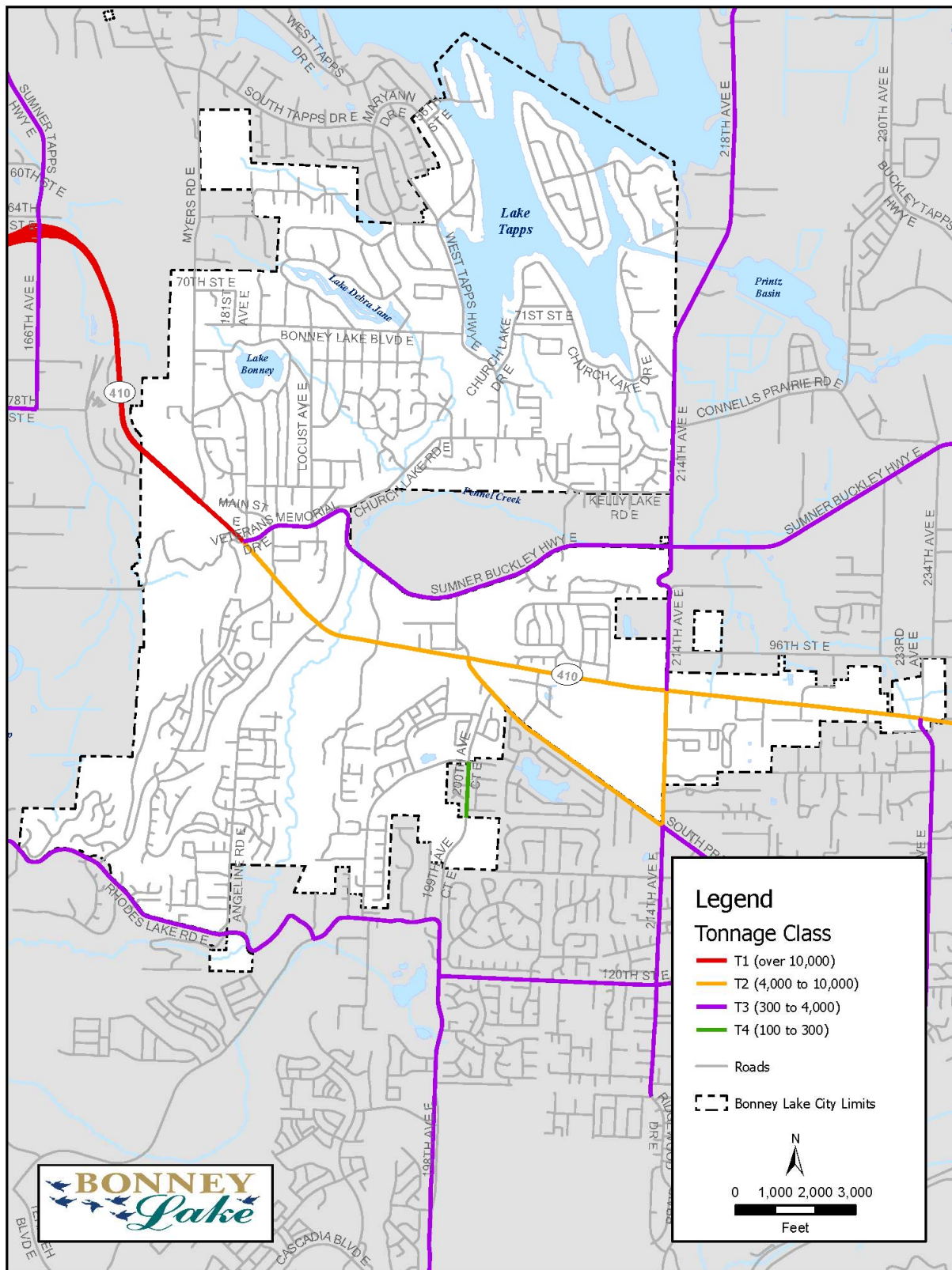
Exhibit 15: Freight and Goods Transportation Classification, City of Bonney Lake, 2025
