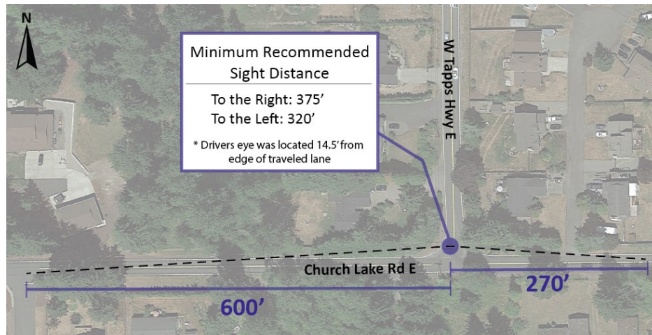
Figure 6. Church Lake Road E at W Tapps Highway Intersection Sight Distance
