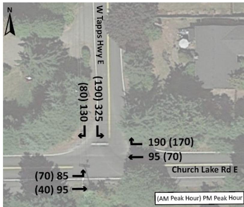
Figure 7. Church Lake Road E at W Tapps Highway 2049 AM and PM Peak Hour Volumes
