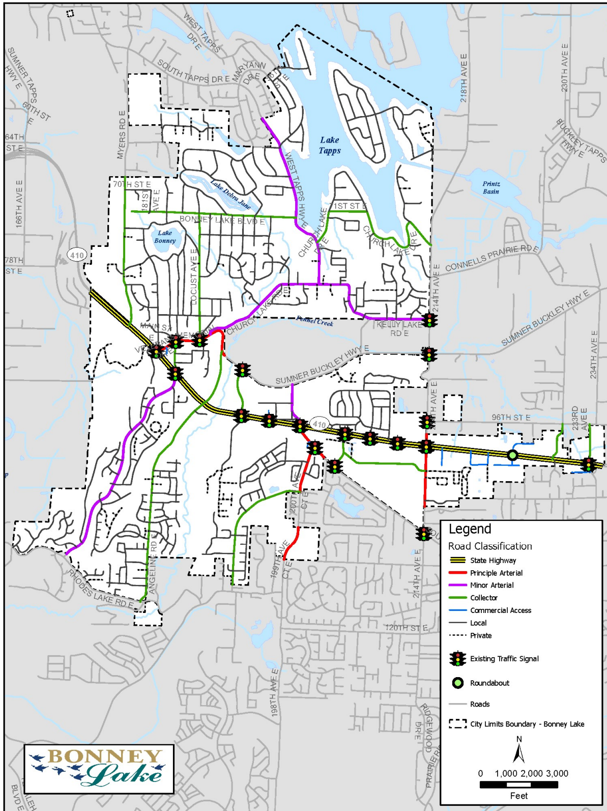
Exhibit 1: Street Functional Classifications and Traffic Signals, 2025
