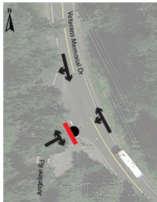
Figure 2. Angeline Road at Veterans Memorial Drive Intersection
