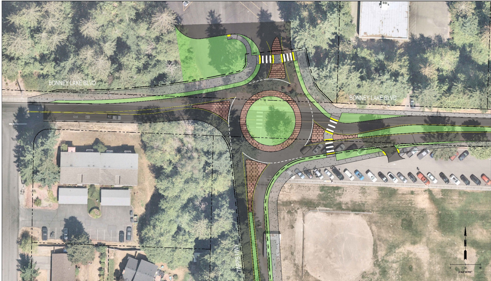
Figure 11. W Tapps Highway at Bonney Lake Boulevard – Proposed Roundabout
