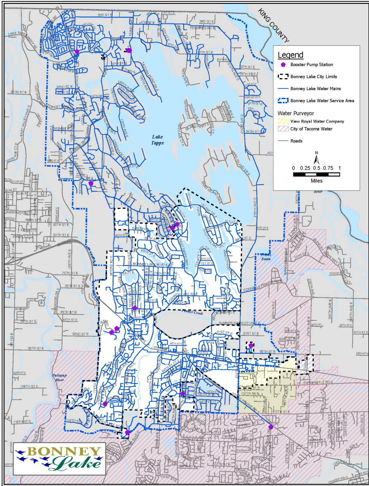
Exhibit 15: City of Bonney Lake Water Infrastructure
