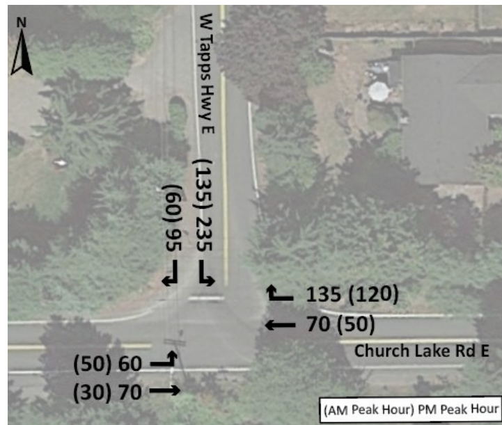
Figure 4. Church Lake Road E at W Tapps Highway 2023 AM and PM Peak Hour Volumes
