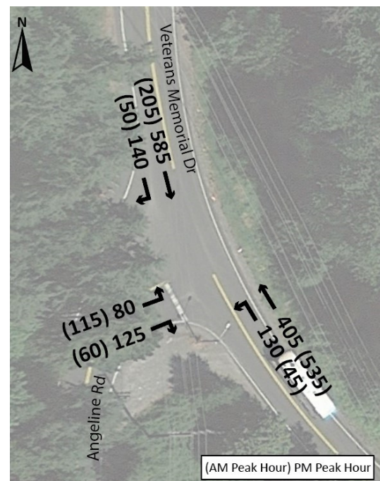
Figure 5. Angeline Road at Veterans Memorial Drive 2023 AM and PM Peak Hour Volumes
