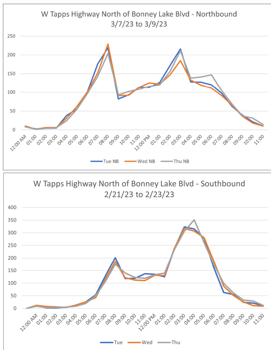
Figure 4. W Tapps Highway North of Bonney Lake Boulevard Hourly Traffic Volumes
