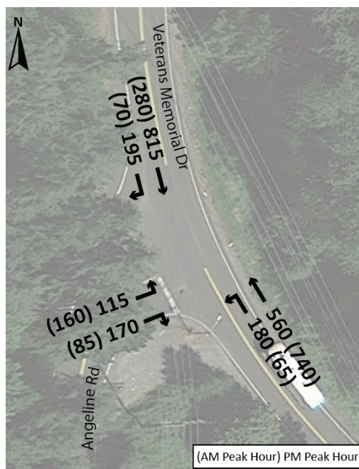
Figure 8. Angeline Road at Veterans Memorial Drive 2049 AM and PM Peak Hour Volumes
