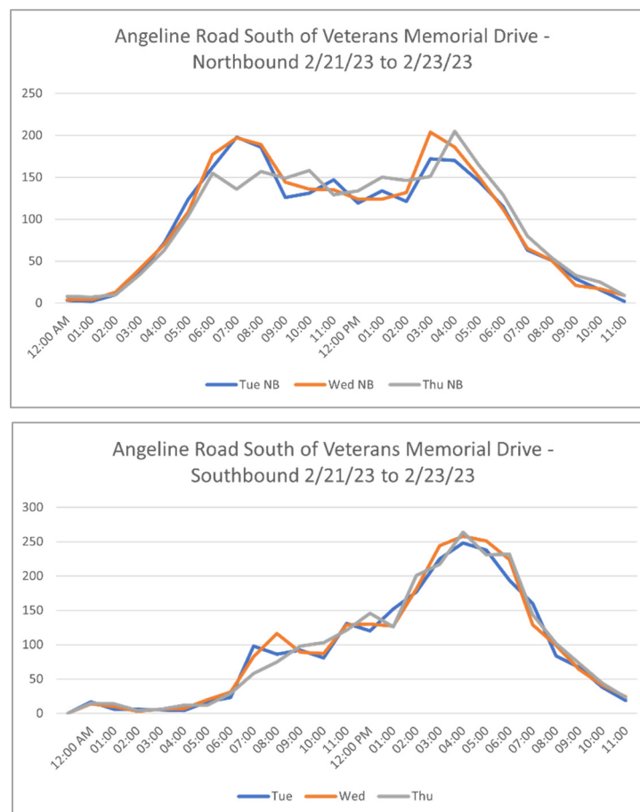
Figure 3. Angeline Road South Veterans Memorial Drive Hourly Traffic Volumes
