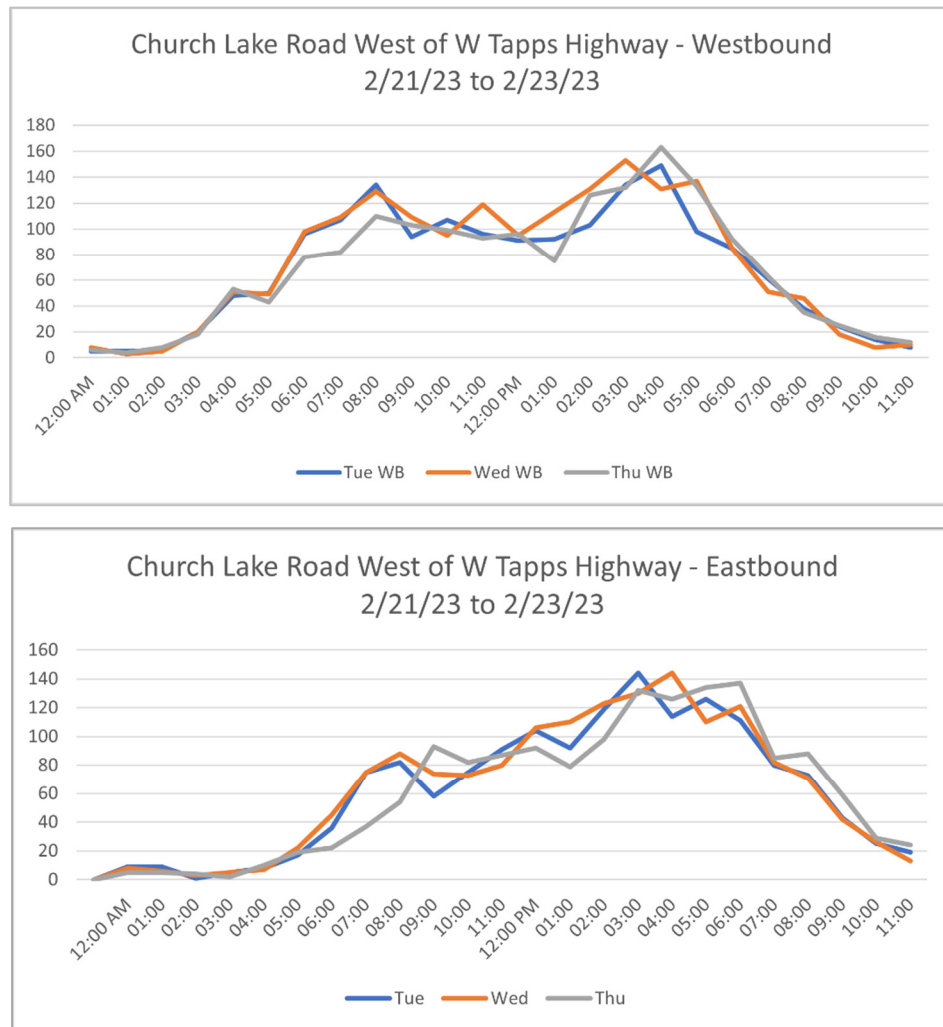
Figure 3. Church Lake Road West of W Tapps Highway Hourly Traffic Volumes
