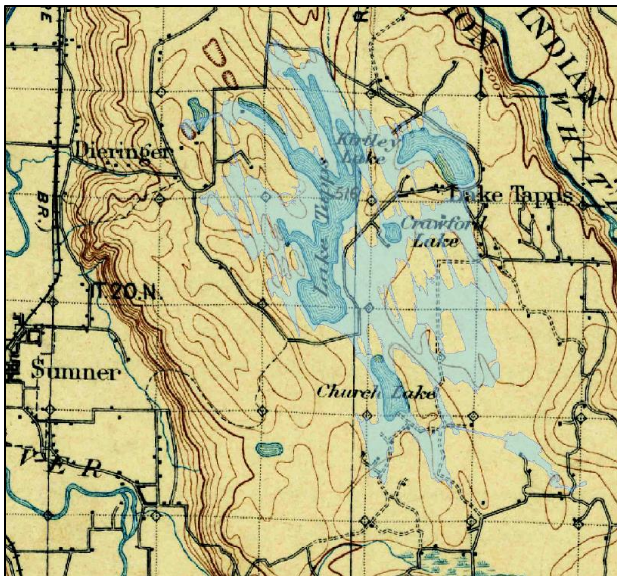
Figure 8-1: The four original lakes as shown on the 1897 USGS Map
