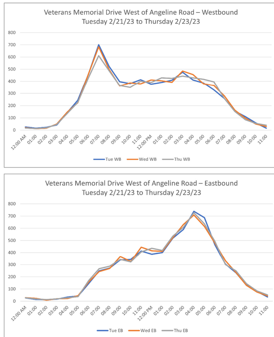
Figure 4. Veterans Memorial Drive West of Angeline Road Hourly Traffic Volumes
