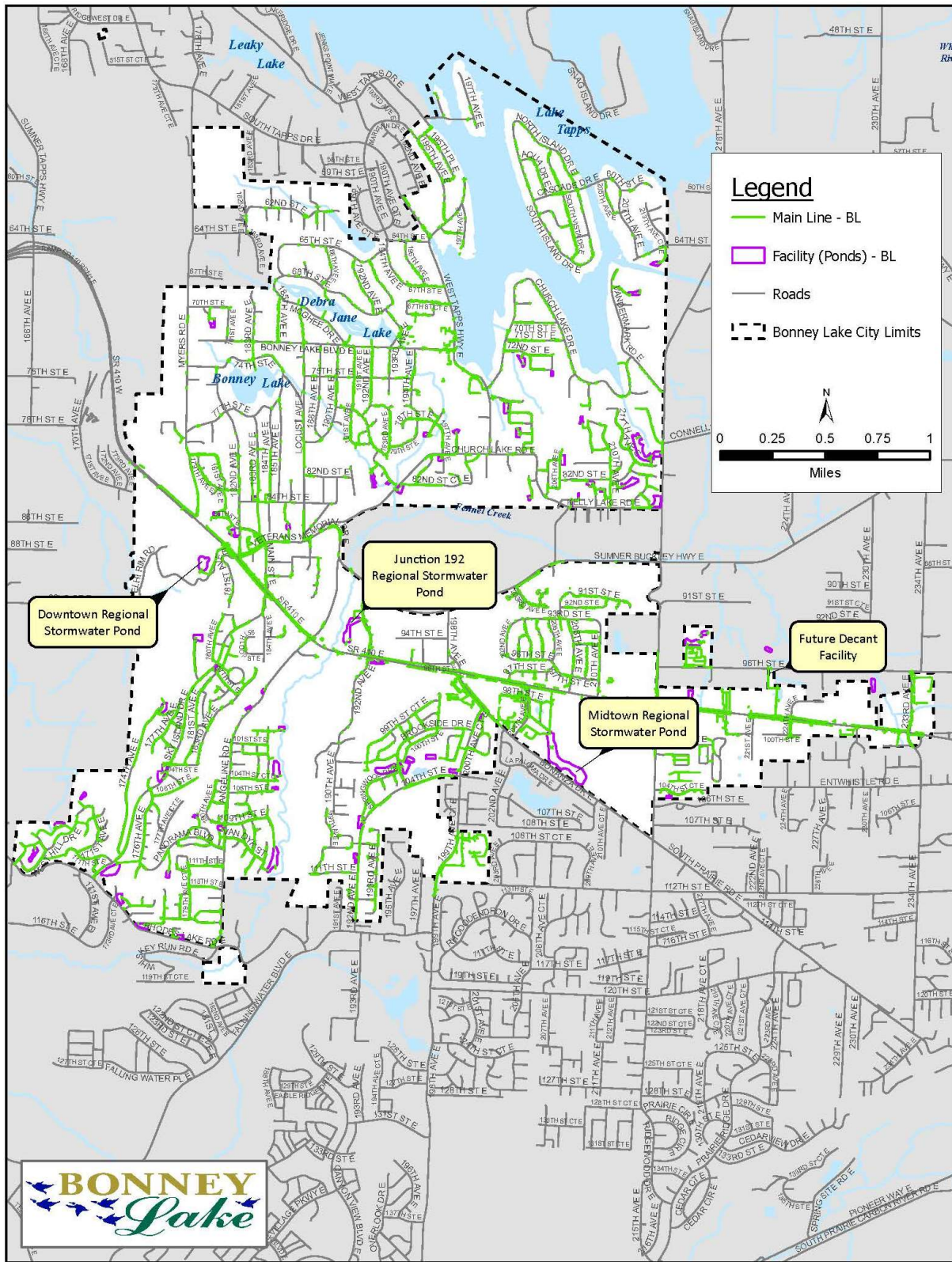
Exhibit 12: City of Bonney Lake Stormwater Facilities, 2025
