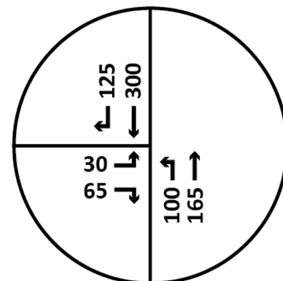
Figure 7. 2023 Summer PM Peak Hour Volumes
