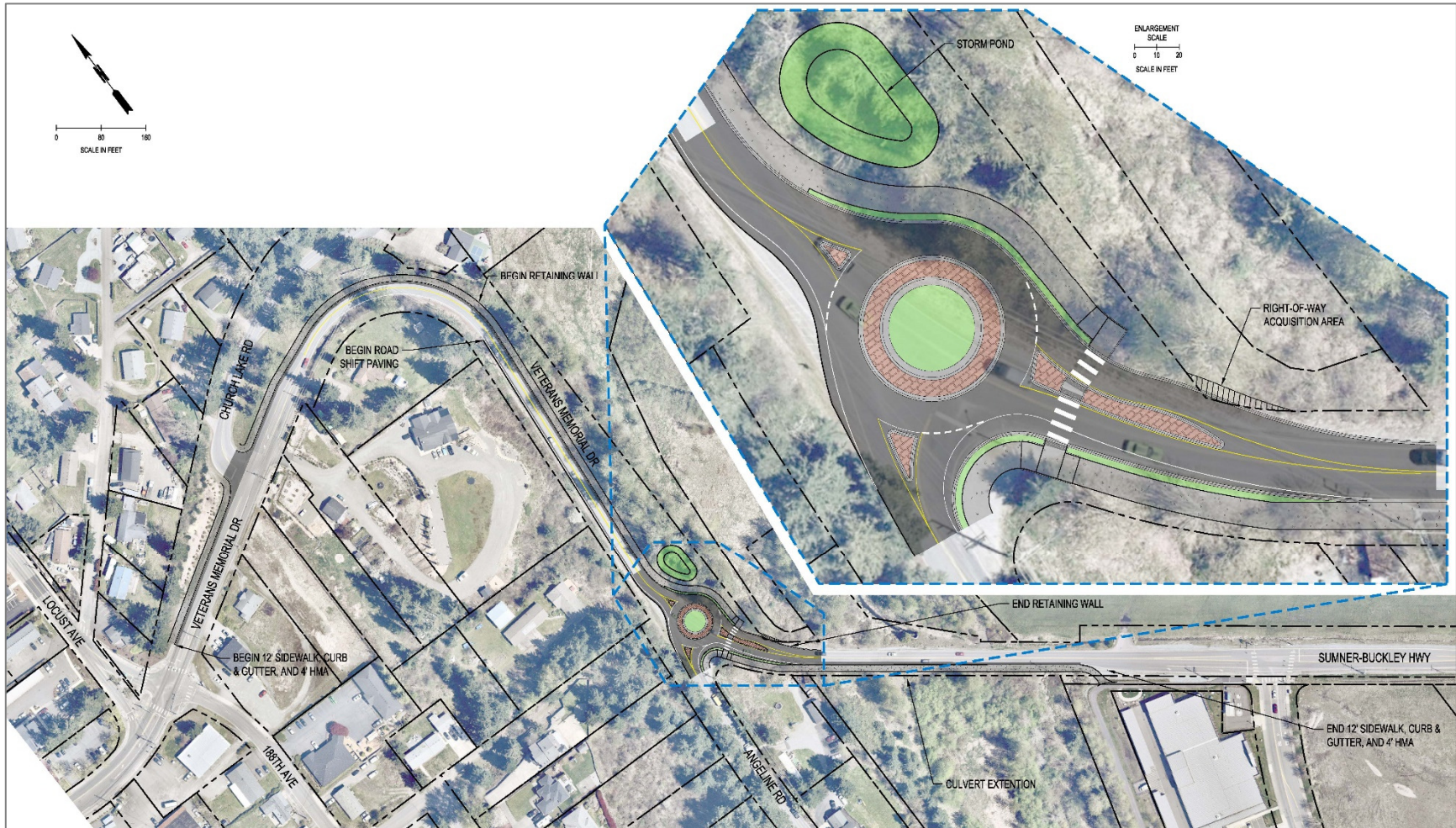
Figure 11. Angeline Road at Veterans Memorial Drive – Roundabout with Shared Use Path
